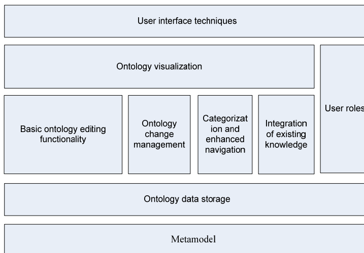
Fig. 3. myOntology components
