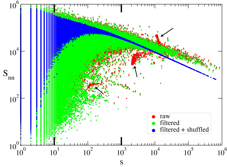
Fig. 14. Average nearest-neighbor strength S_{nn} of nodes (tags) in relation to the node (tag) strengths s , in del.icio.us . Red dots correspond to the whole co-occurrence network. Assortative behavior is observed for low values of the strength s , while disassortative behavior is visible for high values of s . A few clusters (indicated by arrows) stand out from the main cloud of data points. As in Fig. 12, such anomalies correspond to spamming activity and can be removed by filtering out posts containing an excessive number of tags (green dots). In this case, shuffling the tags (blue points) affects dramatically the distribution of data points: this happens because the average nearest-neighbor strength of nodes is able to probe the local structure of the network of co-occurrence beyond the pure frequency effects, and is sensitive to patterns of co-occurrence induced by semantics.
