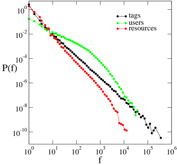
Fig. 4. Probability distribution of the frequency of occurrence of tags, users and resources in del.icio.us. For tags (black dots), the abscissa of each point corresponds to a given frequency, and its ordinate is the fraction of tags that occur with the selected frequency. The same holds for users (green dots) and resources (red dots).
