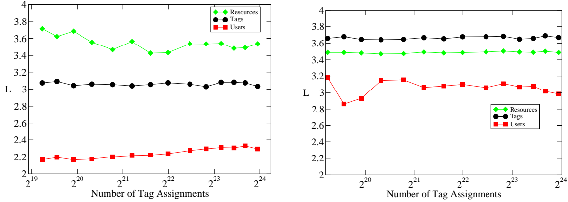
Fig. 9. Characteristic path lengths of delicio.us in the three cooccurrence graphs (left) and in the hypergraph for the three dimensions (right). The left diagram shows the characteristic path lengths of the three cooccurrence graphs in one diagram. The difference reflect the different sizes of the co-occurrence graphs; the larger graphs have higher characteristic path length. The right diagram shows the different contributions of the tags, users, and resources to the delicio.us curve in the right diagrams of Figures 5 and 8. For computing the values, the random nodes have been drawn only from the respective class. The low char. path lengths of the user nodes reflect the structural importance of the personomies in the hyper-graph. The char. path lengths of the tags and resources are reversed compared to the left diagram; indicating that tags tend to be more independent from the core folksonomy structure than resources.
