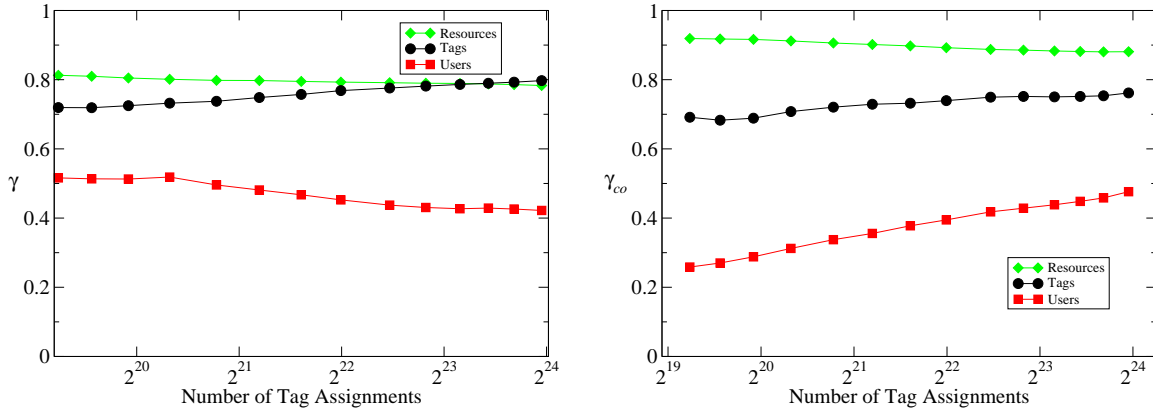
Fig. 10. Clustering coefficient of delicio.us for the three co-occurrence graphs (left) and connectedness of the hypergraph by dimension (right). Both diagrams show that the neighborhoods around tags and resources are denser than around users. The user curve in the left diagram decreases over time, while it increases in the right one.
