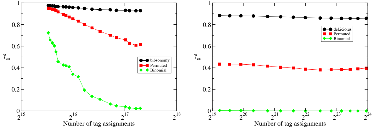
Fig. 7. Connectedness/Transitivity of the BibSonomy folksonomy (left) and the del.icio.us folksonomy (right), compared with the corresponding random graphs: permuted and binomial (see text). The measure is repeated following the network growth and shown as a function of the number of tagging events. Similar graphs have been obtained as a function of the number of nodes of the networks (not shown). As in the case of cliquishness, the values of connectedness/transitivity are very high for the folksonomy networks, at odds with the corresponding random graphs (permuted and binomial).
