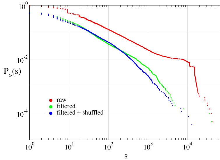
Fig. 13. Cumulative strength distribution P_{>}(s) for the network of co-occurrence of tags in BibSonomy (see also Fig. 12). Red dots correspond to the whole co-occurrence network. The irregular behavior for high strengths can be linked to spamming activity: identified spam in BibSonomy consists of posts with a large number of tags, as well as a large number of posts with exactly 10 tags, injected by a small group of spammers. Both types of spam were identified by inspecting the distribution of the number of tags per post. Excluding the above posts from the analysis (green dots), the distribution becomes smooth and similar to the filtered one observed for del.icio.us. Similarly, shuffling the tags contained in posts (blue dots) has a small effect on the cumulated weight distribution.
