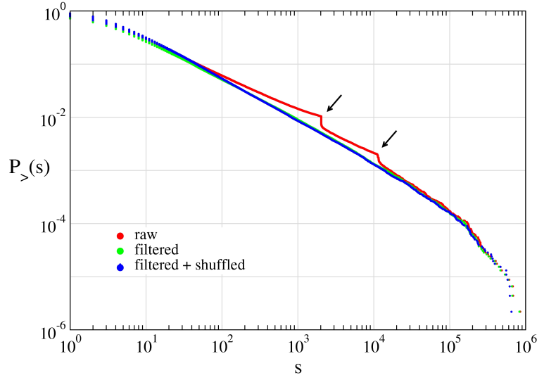
Fig. 12. Cumulative strength distribution for the network of co-occurrence of tags in del.icio.us. P_{>}(s) is the probability of having a node with strength in excess of s . Red dots correspond to the whole co-occurrence network. The two steps indicated by arrows correspond to an excess of links with a specific weight and can be related to spamming activity. Excluding from the analysis all posts with more than 50 tags removes the steps (green dots). Shuffling the tags contained in posts (blue dots) does not affect significantly the cumulated weight distribution. This proves that such a distribution is uniquely determined by tag frequencies within the folksonomy, and not by the semantics of co-occurrence.
