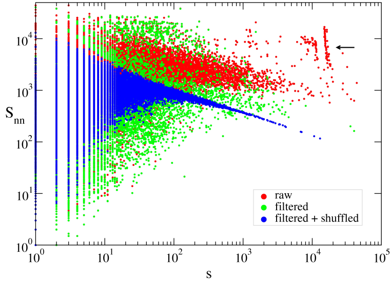
Fig. 15. Average nearest-neighbor strength S_{nn} of nodes (tags) in relation to the node (tag) strengths s , in BibSonomy . Red dots correspond to the whole co-occurrence network. The scatter plot is qualitatively very similar to the one reported in Fig. 14 for del.icio.us : assortative behavior is observed for low values of the strength s , while disassortative behavior is visible for high values of s . Again, a few clusters (indicated by arrows) stand out from the main cloud of data points and their presence can be linked to spamming activity. They disappear when we filter out posts containing an excessive number of tags (green dots). Shuffling the tags (blue dots) has the same effect as in Fig. 14, and the same observations apply.
