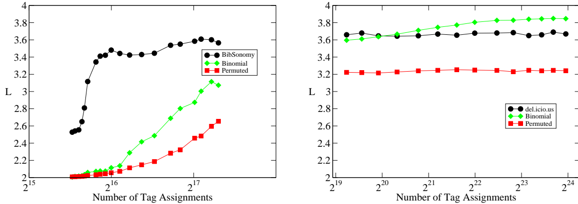
Fig. 8. Characteristic path length L considering only tags in BibSonomy (left) and del.icio.us (right). The figures show that the characteristic path length restricted to tags is almost constant starting from a very early point in the growth of the folksonomy.
