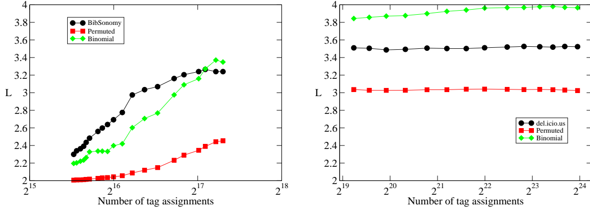
Fig. 5. Characteristic path length for the BibSonomy folksonomy (left) and the del.icio.us folksonomy (right), compared with the corresponding random graphs: permuted and binomial (see text). The measure is repeated following the network growth and shown as a function of the number of tagging events. Similar graphs have been obtained as a function of the number of nodes of the networks (not shown). Note how the characteristic path length takes quite similar low values, typical of small world networks, for all graphs.
