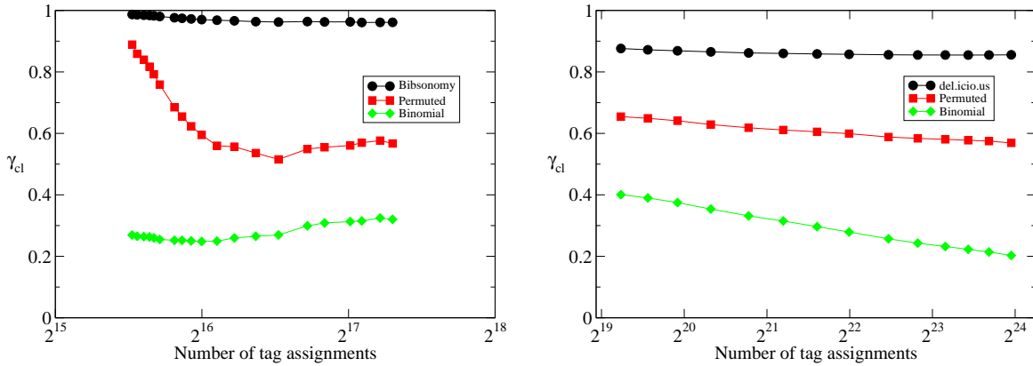
Fig. 6. Cliquishness of the BibSonomy folksonomy (left) and the del.icio.us folksonomy (right), compared with the corresponding random graphs: permuted and binomial (see text). The measure is repeated following the network growth and shown as a function of the number of tagging events. Similar graphs have been obtained as a function of the number of nodes of the networks (not shown). The cliquishness for the folksonomy networks takes quite high values, higher than the corresponding random graph (permuted and binomial).
