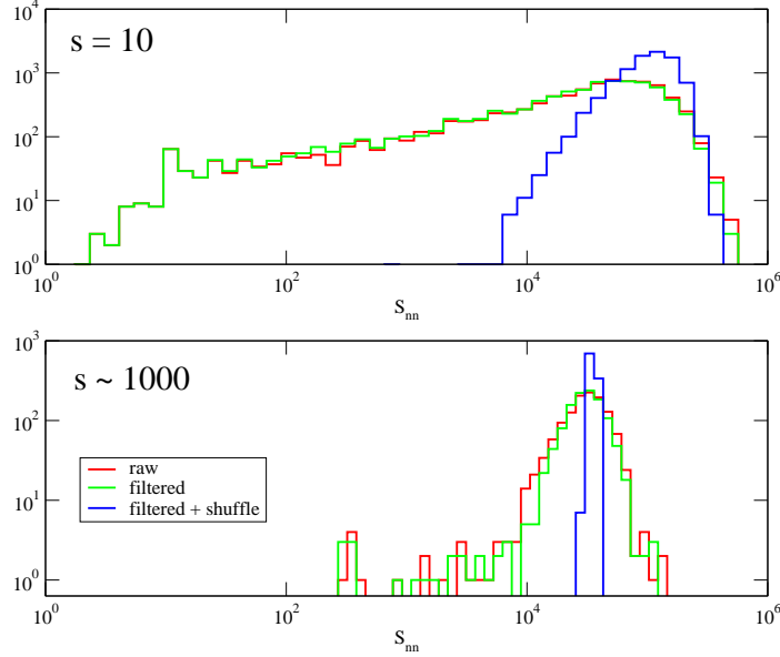
Fig. 16. Histograms of the average nearest-neighbor strength S_{nn} of nodes having a value of node strength s , in delicio.us . The data are extracted from the scatter plot of Fig. 14 for two values of the strength, i. e., s = 10 (upper panel) and s = 1000 (lower panel). The two values of the strength are chosen in order to show more clearly the whole distribution of scattered points in two qualitatively different regions of Fig. 14. The two regions are only slightly affected by spam. In the upper panel ( s = 10 ) a broad distribution appears, characterized by a most probable high value of S_{nn} and a broad algebraic tail for smaller values. Interestingly, shuffling the tags dramatically changes the distribution and the tail disappears, indicating that the tail behavior is not a trivial frequency effect. In the lower panel ( s = 1000 ) the tail is narrower, but the shuffling procedure gives qualitatively the same result.
