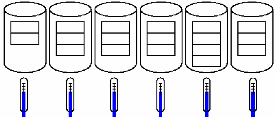
Greedy-Methode
