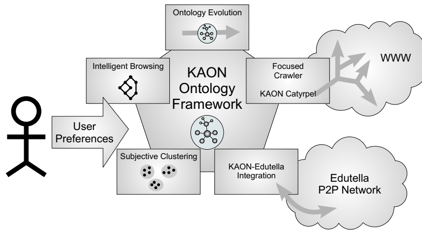
Fig. 2. The components of the Courseware Watchdog.
