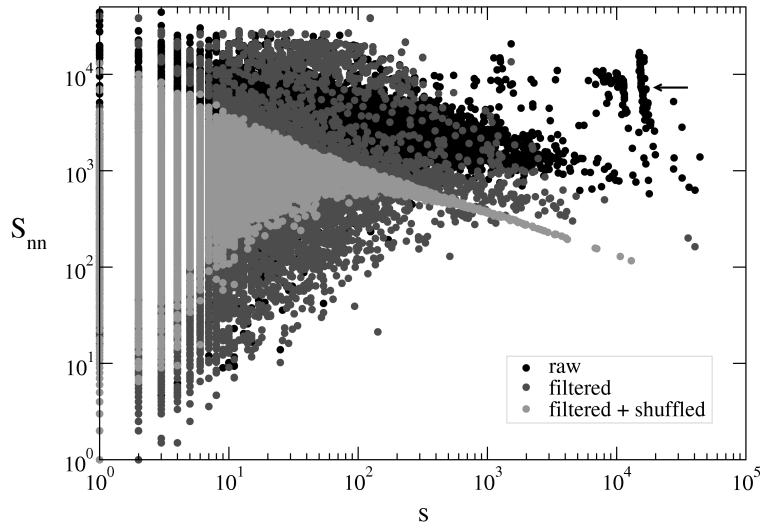
Fig. 15. Average nearest-neighbor strength S_{nn} of nodes (tags) in relation to the node (tag) strengths s , in BibSonomy. Black dots correspond to the whole co-occurrence network. The scatter plot is qualitatively very similar to the one reported in Fig. 14 for del.icio.us: assortative behavior is observed for low values of the strength s , while disassortative behavior is visible for high values of s . Again, a few clusters (indicated by arrows) stand out from the main cloud of data points and their presence can be linked to spamming activity. They disappear when we filter out posts containing an excessive number of tags (dark grey). Shuffling the tags (light gray) has the same effect as in Fig. 14, and the same observations apply.
